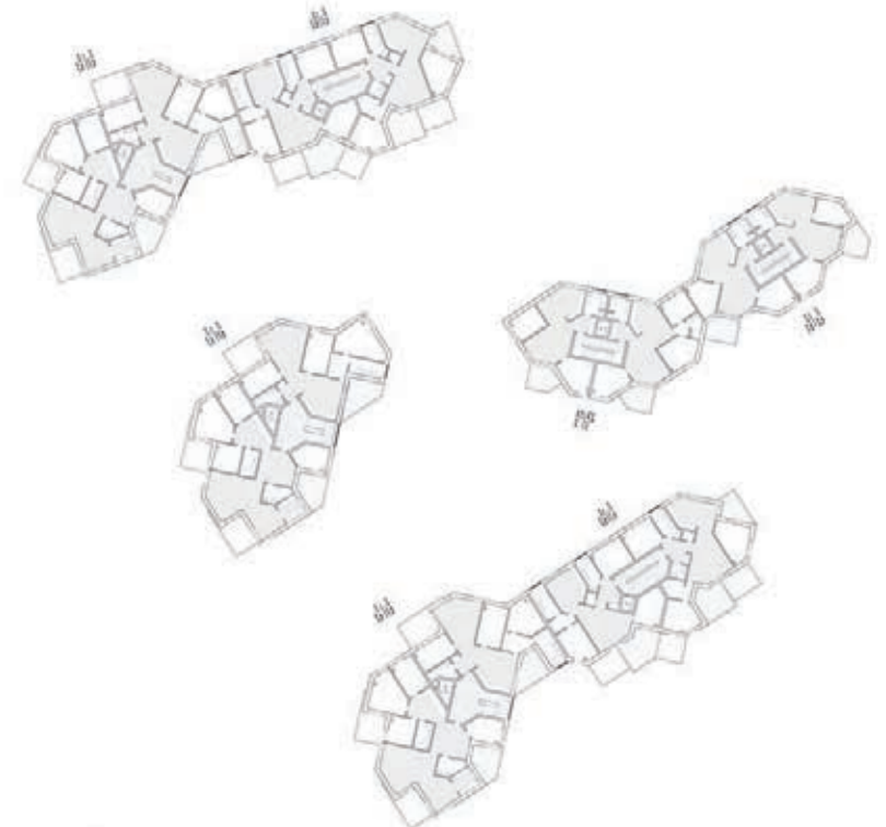
Grundriss Attikageschoss 1:1000
